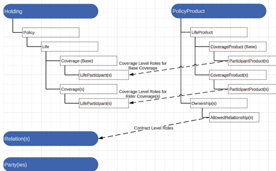
Correlation between Product and Holding for Life Insurance
