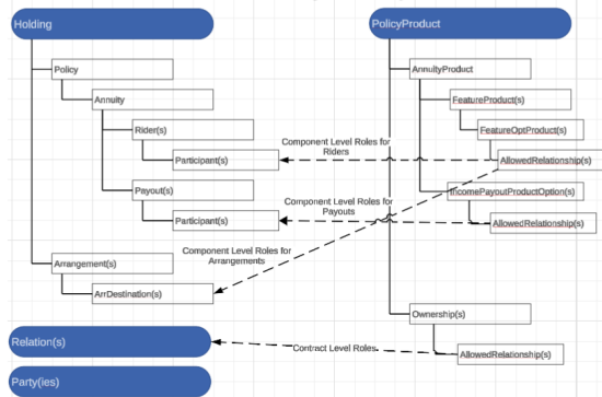
Correlation between Product and Holding for Annuity
